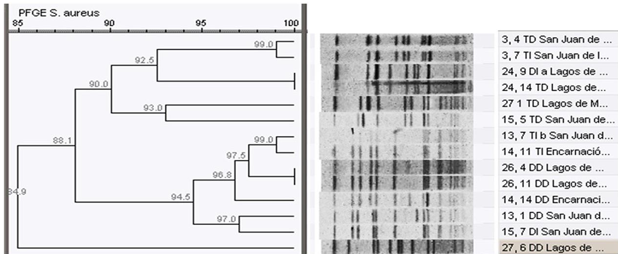
Figure 3. Pulsotype dendrogram of 14 isolated S. aureus strains in the Altos Norte region from Jalisco state
