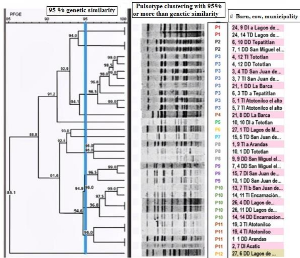
Figure 2. Pulsotype dendrogram of 32 S. aureus isolated strains in different regions from Jalisco state
