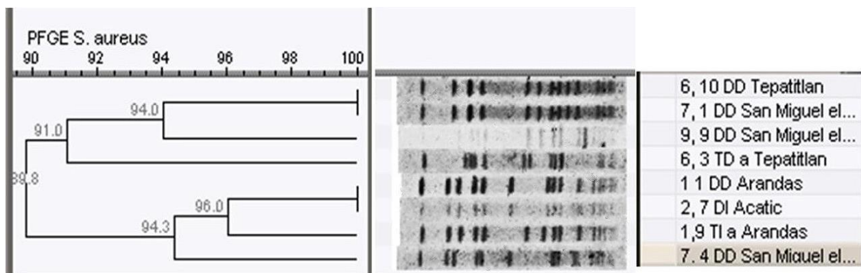
Figure 4. Pulsotypes dendrogram of 8 isolated S. aureus strains in Altos Sur region from Jalisco state
