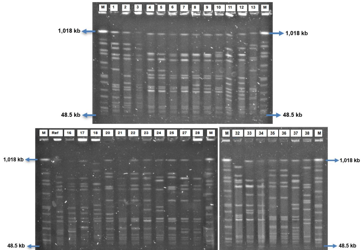
Figure 1. Pulsed field electrophoresis of DNA (after digestion with the restriction enzyme smaI ) of the 32 isolated S. aureus strains from dairy cows in Jalisco state. Where M = Molecular weight marker from 48.5kb to 1,018kb (New England Biolabs), Ref = S. aureus reference strain (ATCC 25923) and number from 1 to 38 = the total number of isolates (32).
